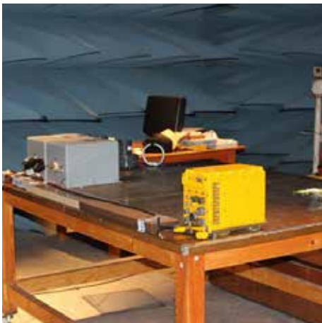
THE CM-ATR-3U PASSES ELECTROMAGNETIC IMMUNITY TEST. CONDUCTED SUSCEPTIBILITY DAMPED SINUSOIDAL TRANSIENTS, CABLES AND POWER LEADS 10 KHz to 100 MHz. MIL-STD-461F CERTIFICATE AVAILABLE.
