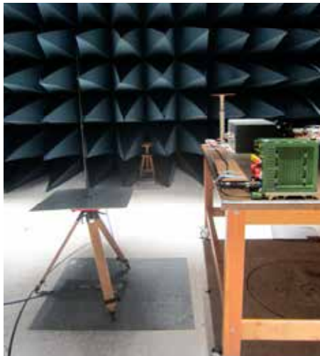
THE CM-ATR-3U PASSES ELECTROMAGNETIC EMISSION & RADIATION TEST. RADIATED E FIELD 2 MHz to 30 MHz. MIL-STD-461F CERTIFICATE AVAILABLE.
